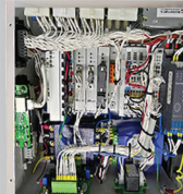
Master Controller
